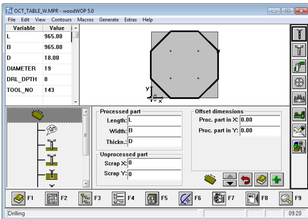
Nesting - WoodWop editor
